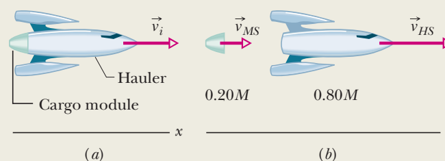
Figure 9-12 (a) A space hauler, with a cargo module, moving at initial velocity \vec{v}_i . (b) The hauler has ejected the cargo module. Now the velocities relative to the Sun are \vec{v}_{MS} for the module and \vec{v}_{HS} for the hauler.
